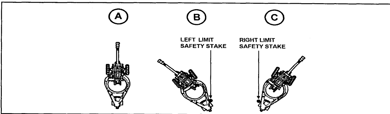
Figure 11-1. Establishment of M119A1 safety limits
