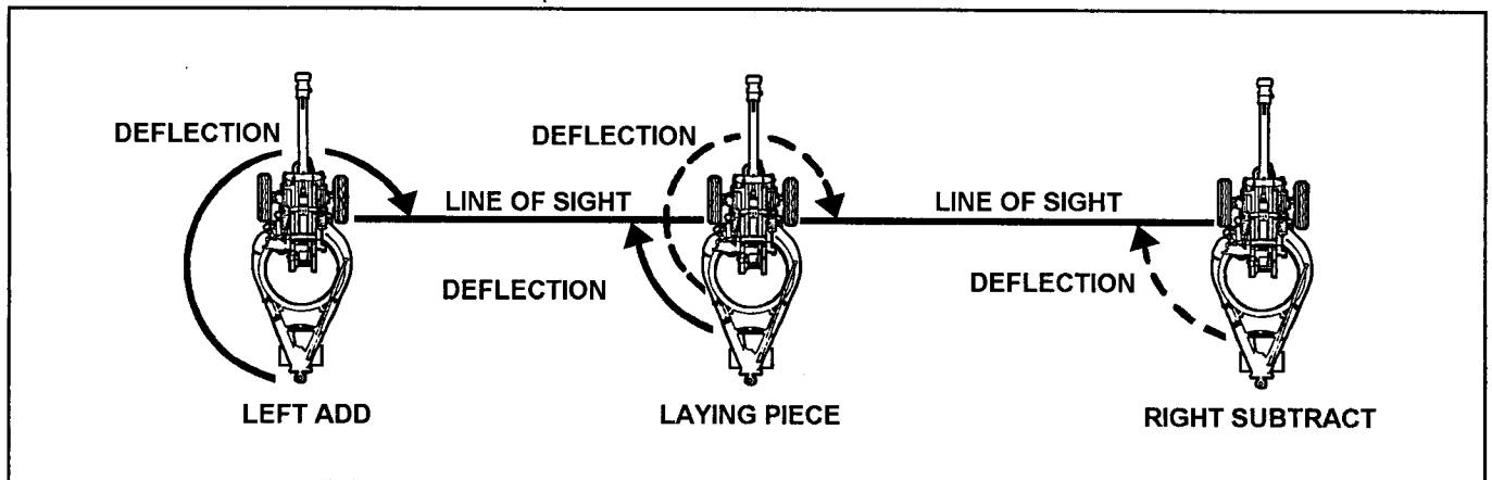
Figure 4-13. Reciprocal laying from another howitzer (M100-series sight)
