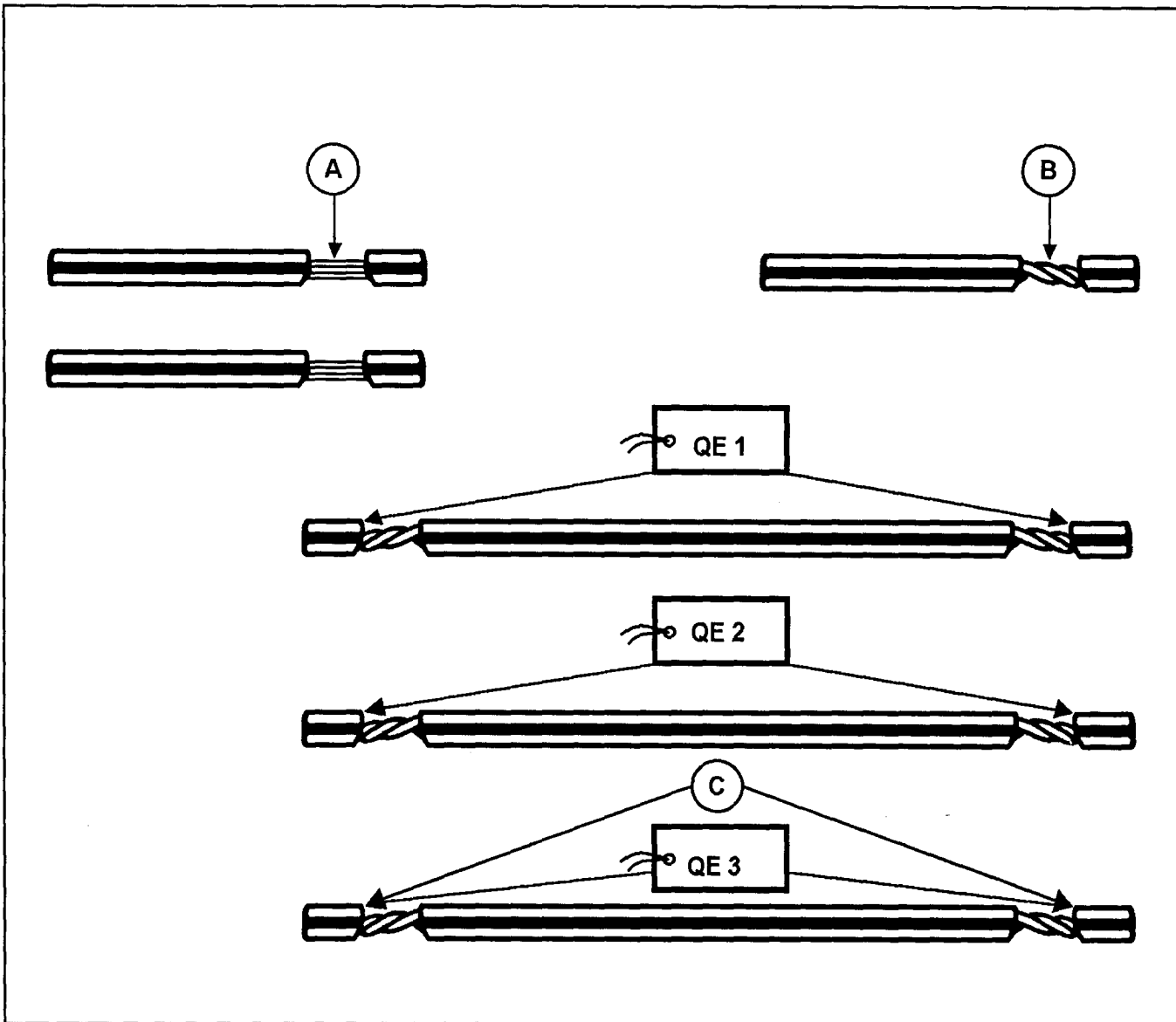
Figure L-8. Preparing wire connector
