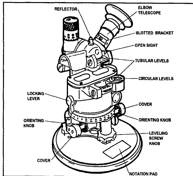
Figure 4-2. Aiming circle (left side view)
