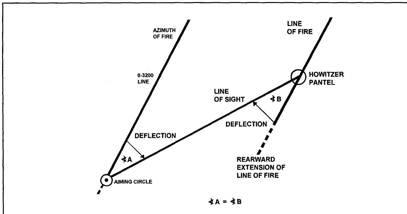
Figure 4-12. Principles of reciprocal laying
