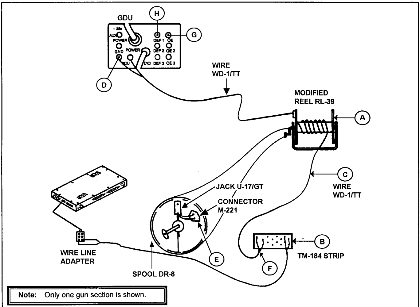
Figure L-7. Connecting the tactical communications interface module and line wire adapter
