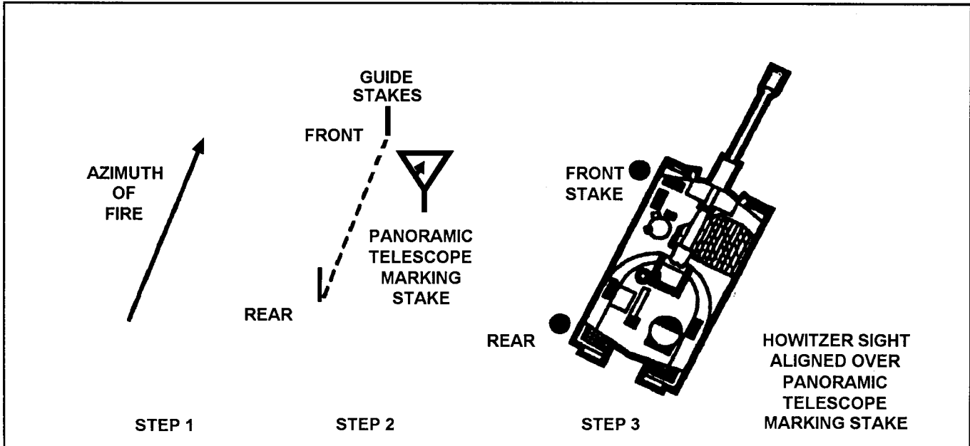
Figure 2-5. Use of stakes for self-propelled weapons
