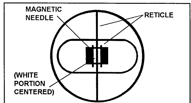
Figure 4-7. Centering the magnetic needle
