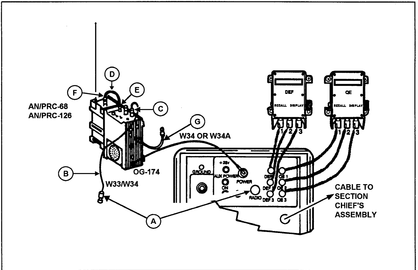
Figure L-16. Gun section cabling for howitzer sections
