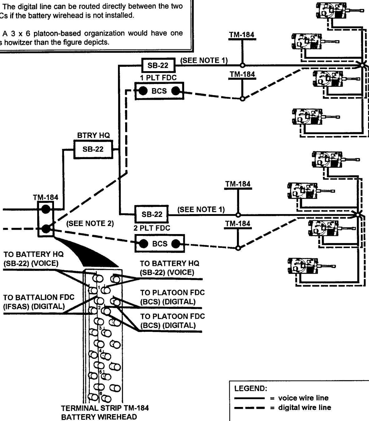
Figure 9-5. Platoon-based battery wire system
