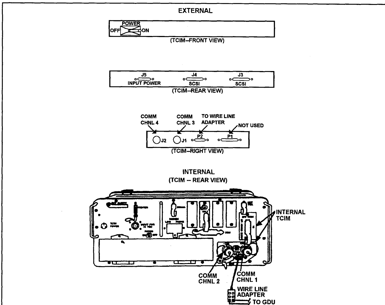
Figure 9-4. Wire and radio connections to the LCU
