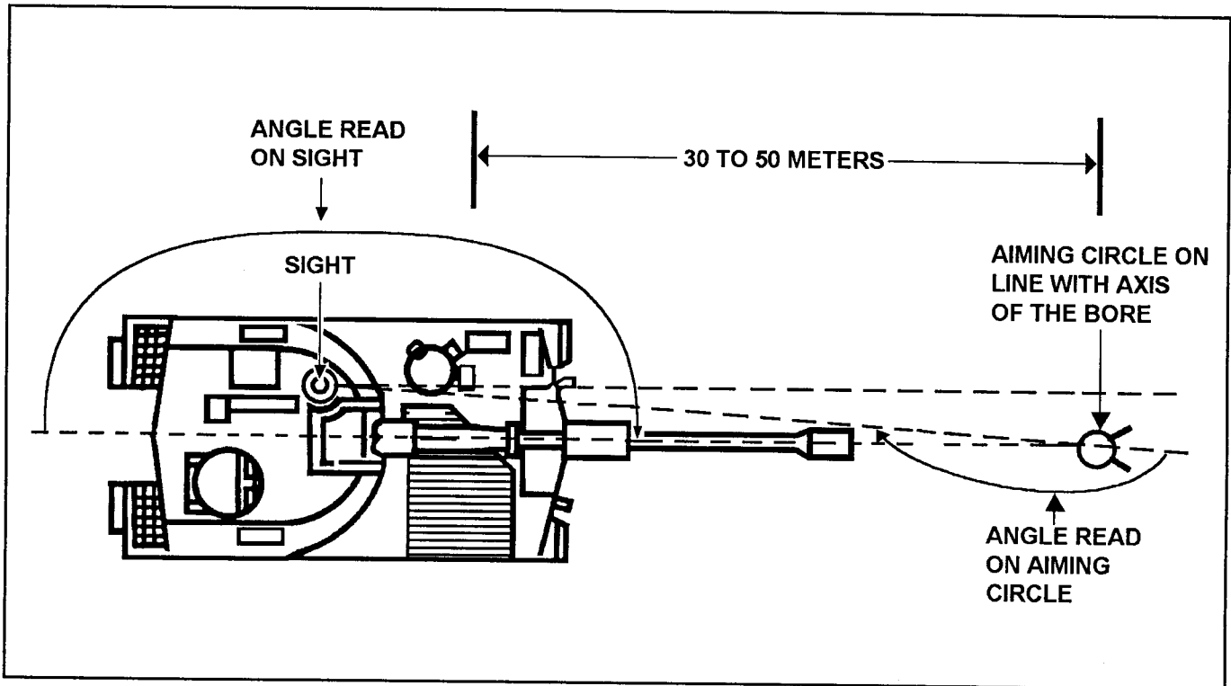
Figure 8-3. Aligning the sight parallel to the axis of the bore by use of an aiming circle
