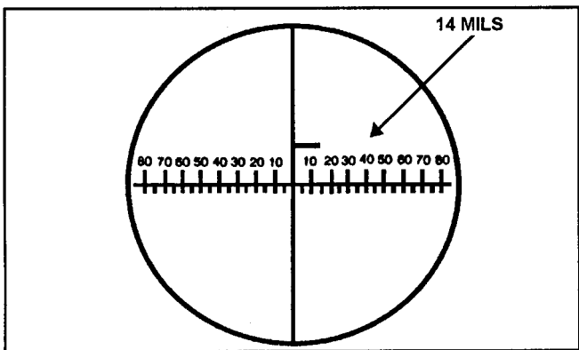
Figure D-1. Aiming post sight picture at 100 meters
