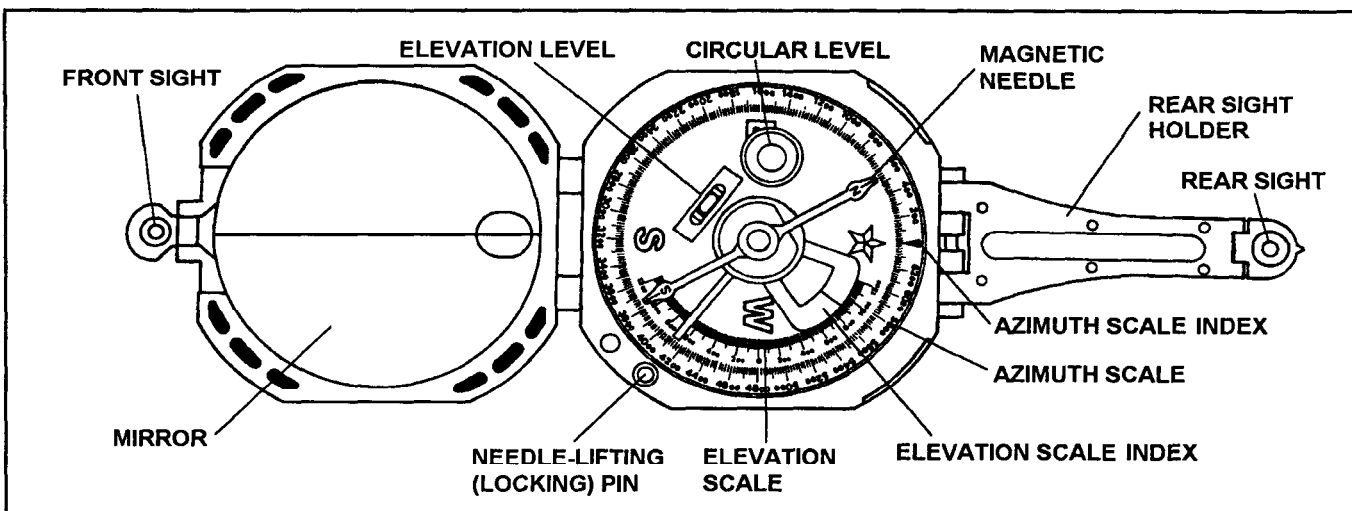
Figure 4-10. M2 compass, top view
