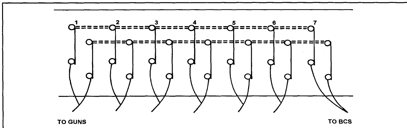
Figure L-6. M-184 terminal strip
