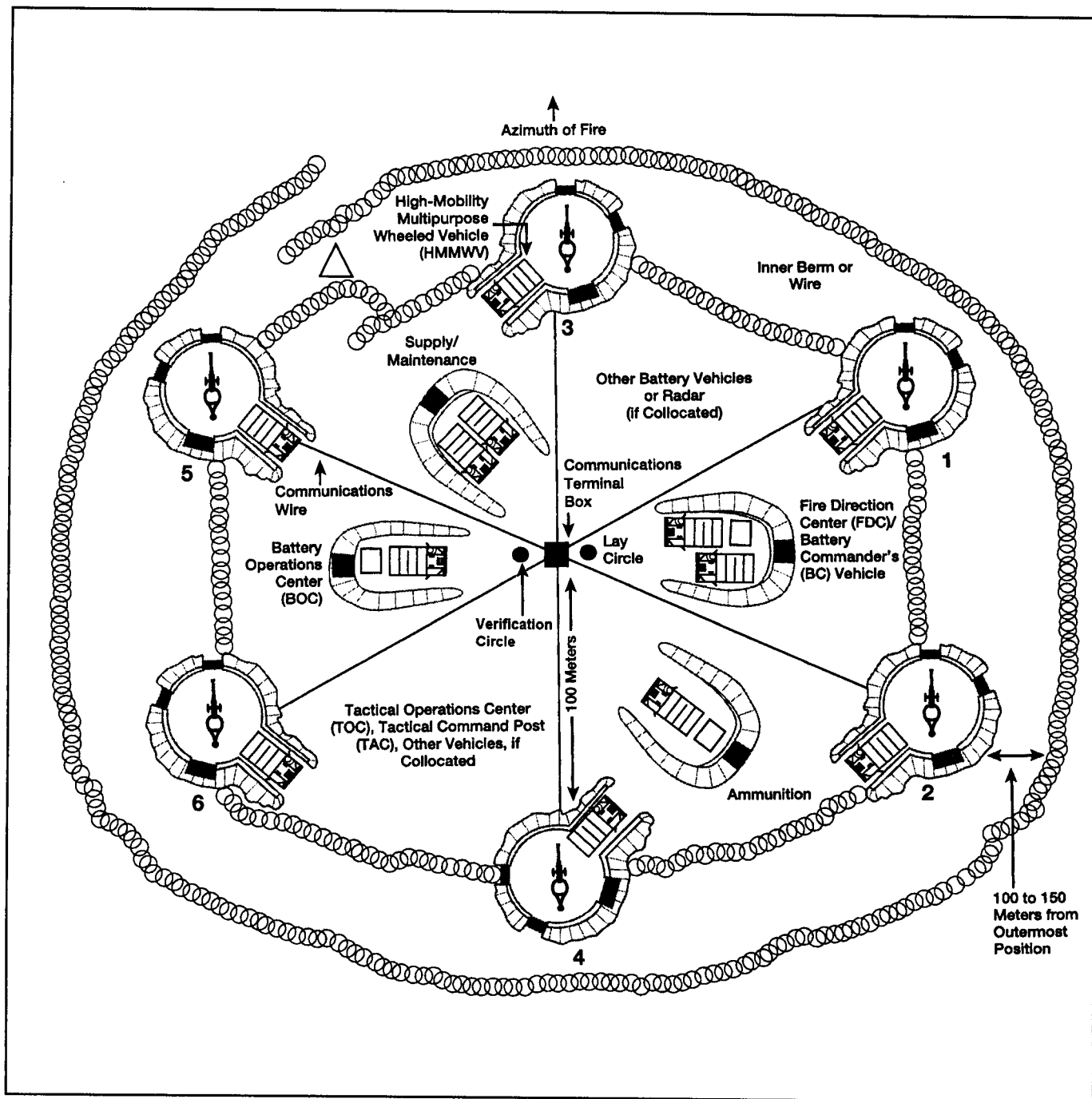
Figure F-1. Hardened battery position in star formation
