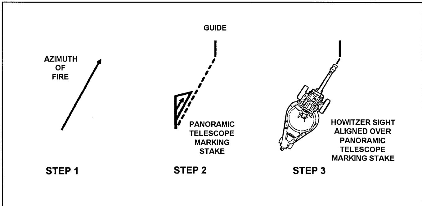
Figure 2-5. Use of stakes for towed weapons
