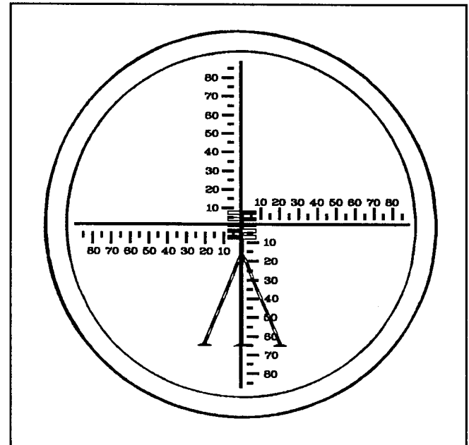
Figure 4-6. Proper sight picture
