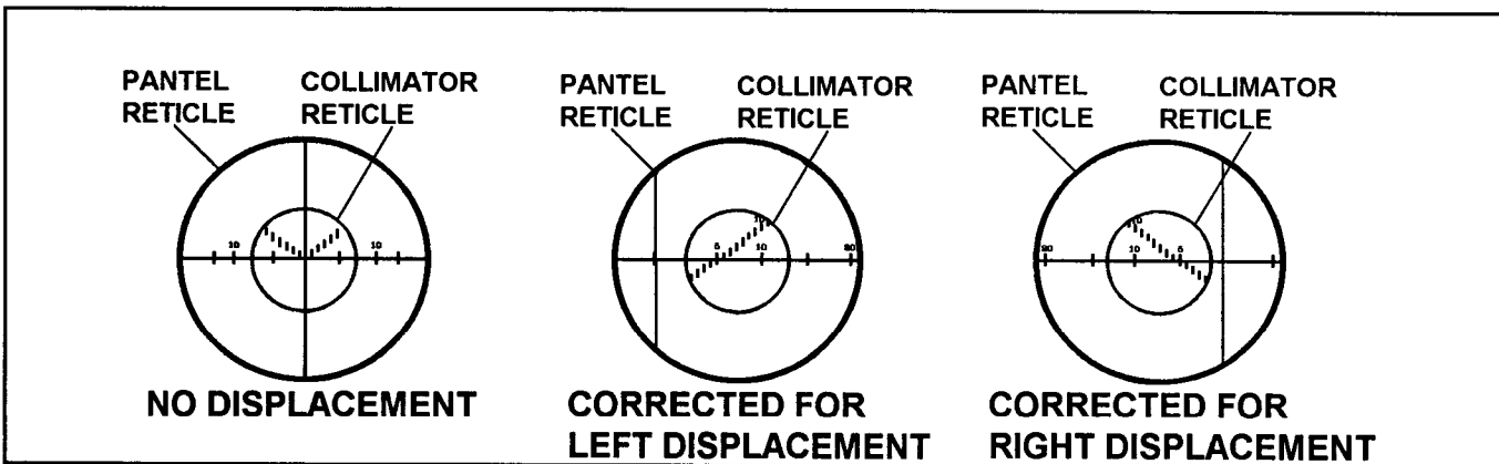
Figure 4-17. Proper sight picture from the weapon
