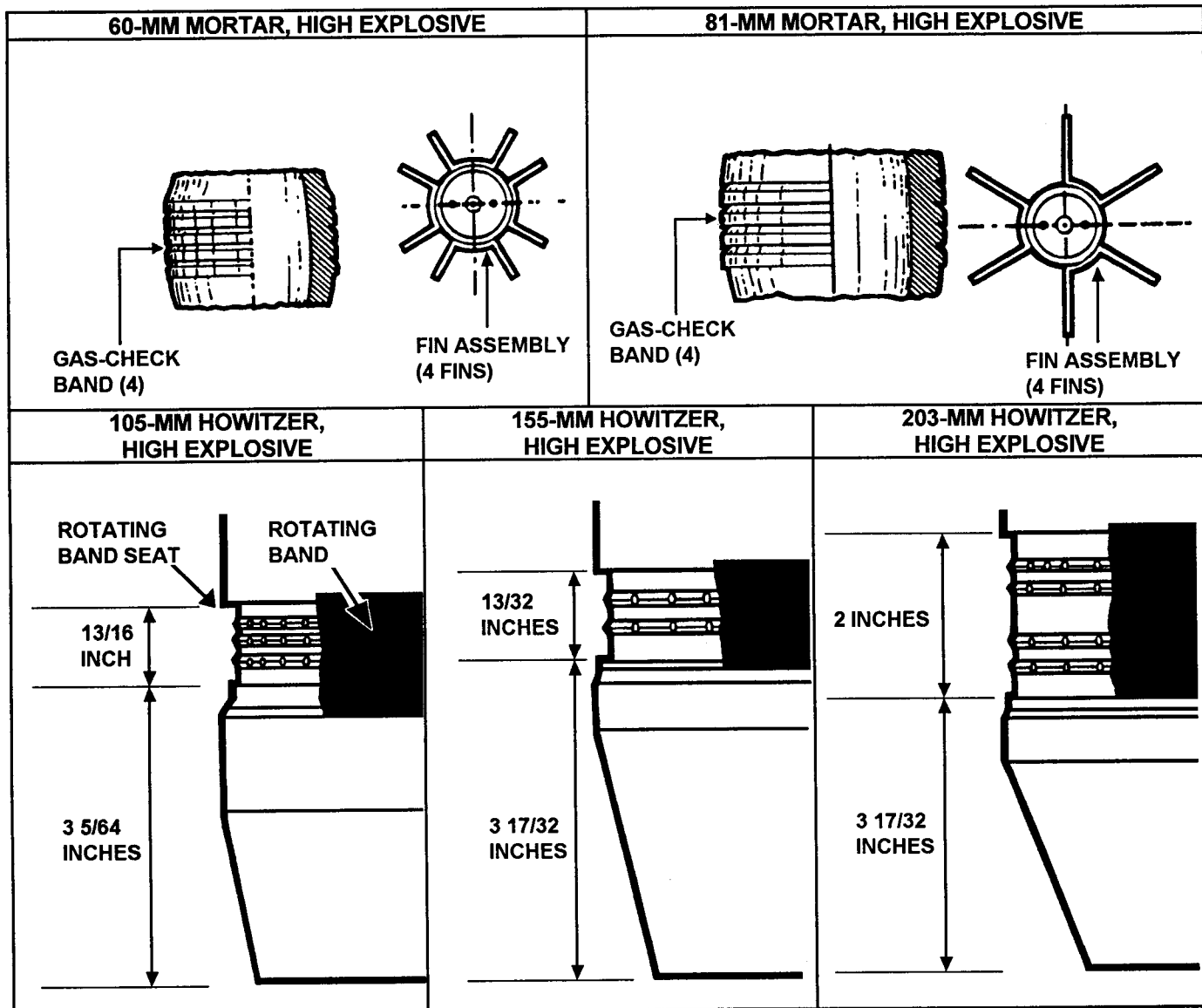
Figure J-9. Shell fragment and tail identification, US ammunition
