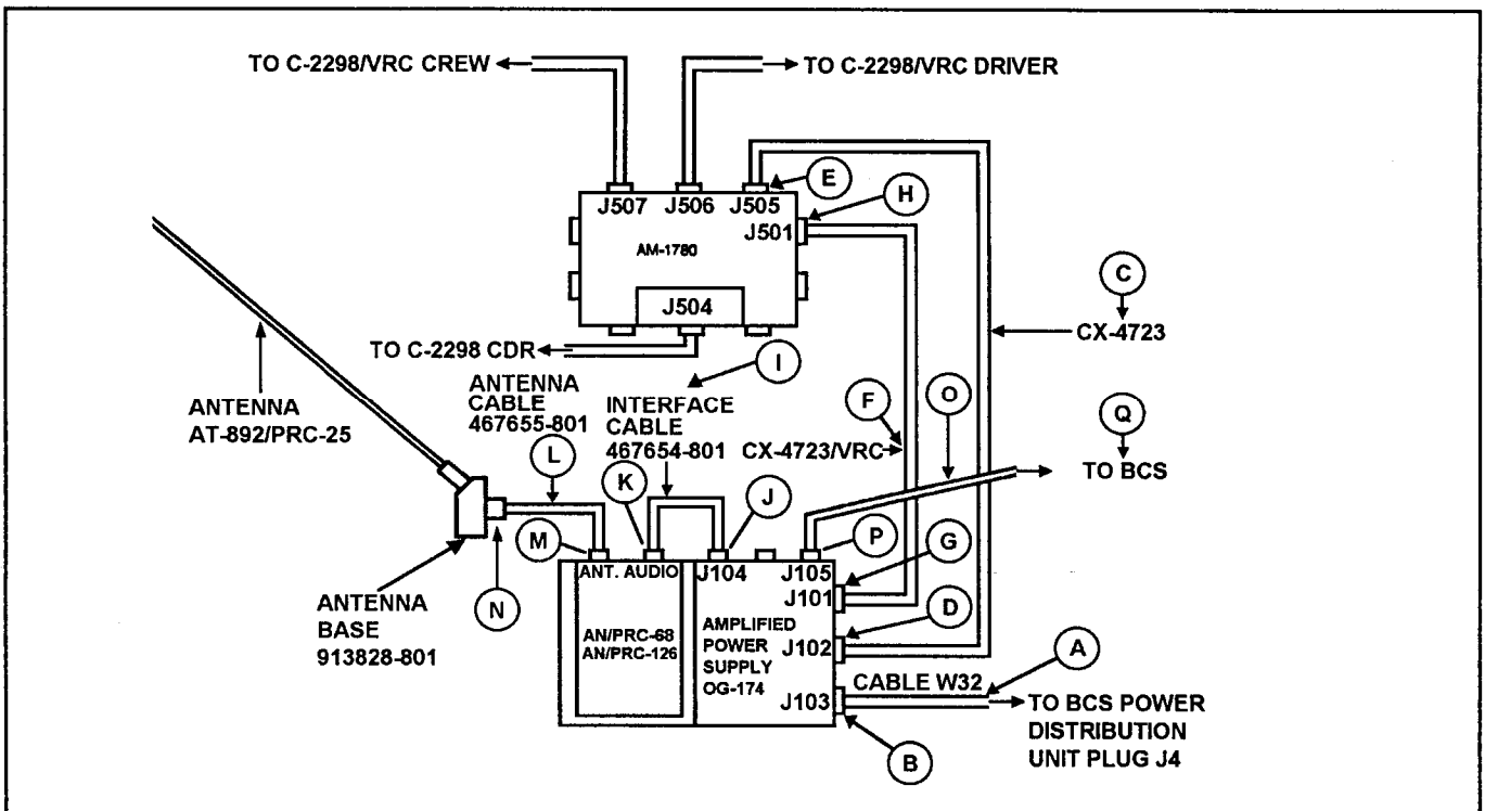
Figure L-15. FDC cabling for the AN/PRC-68 or AN/PRC-126
