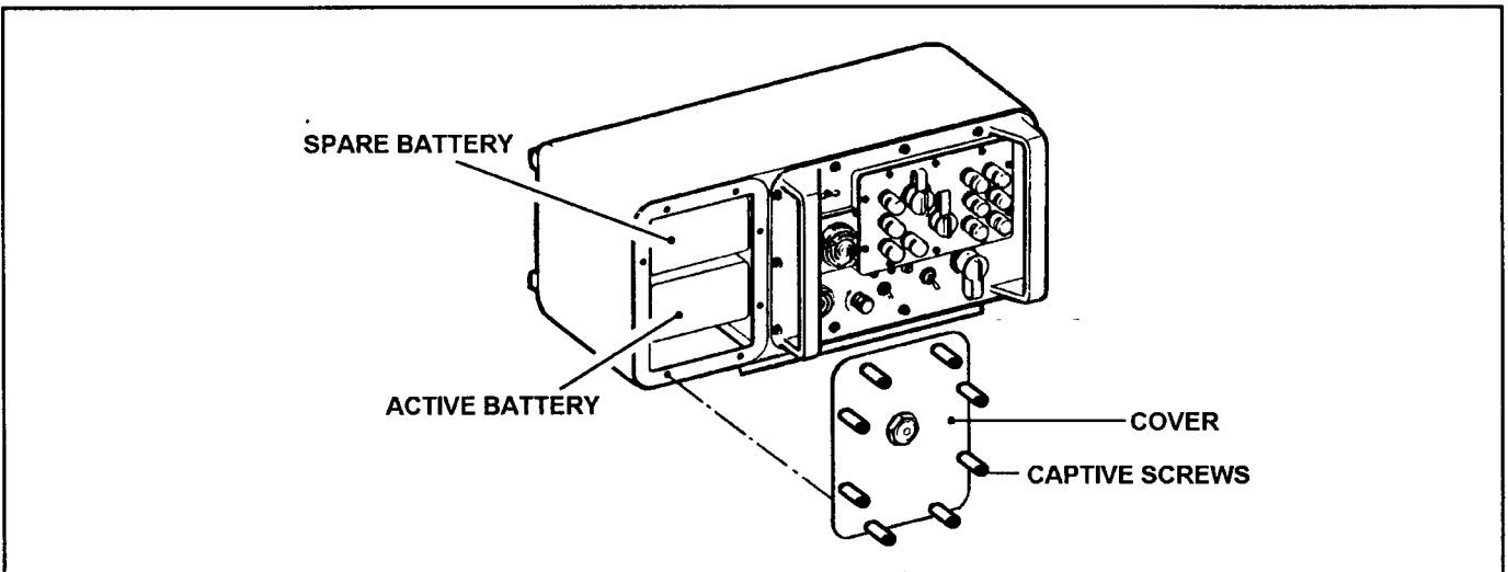
Figure L-10. Battery installation in the case assembly
