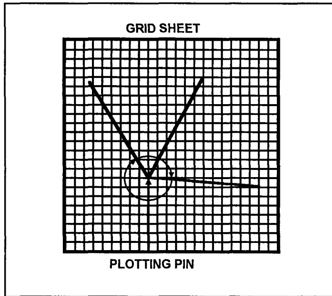
Figure 5-10. Determining position
