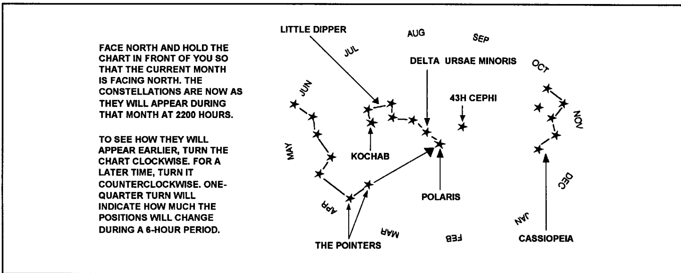
Figure 5-2. Star locations
