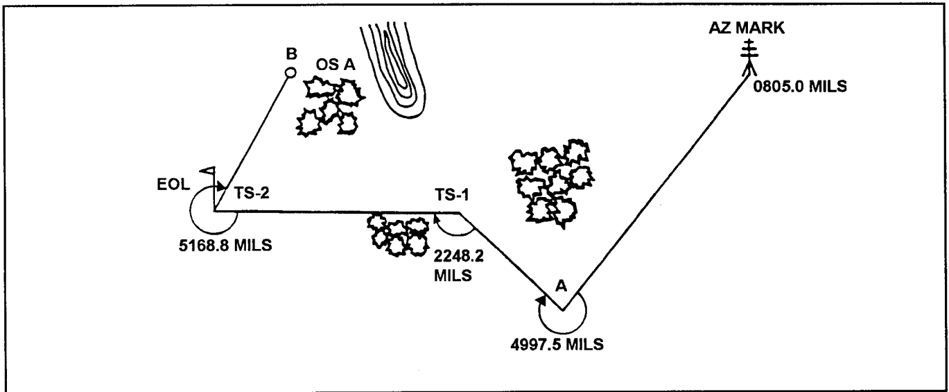
Figure 5-7. Example of a directional traverse
