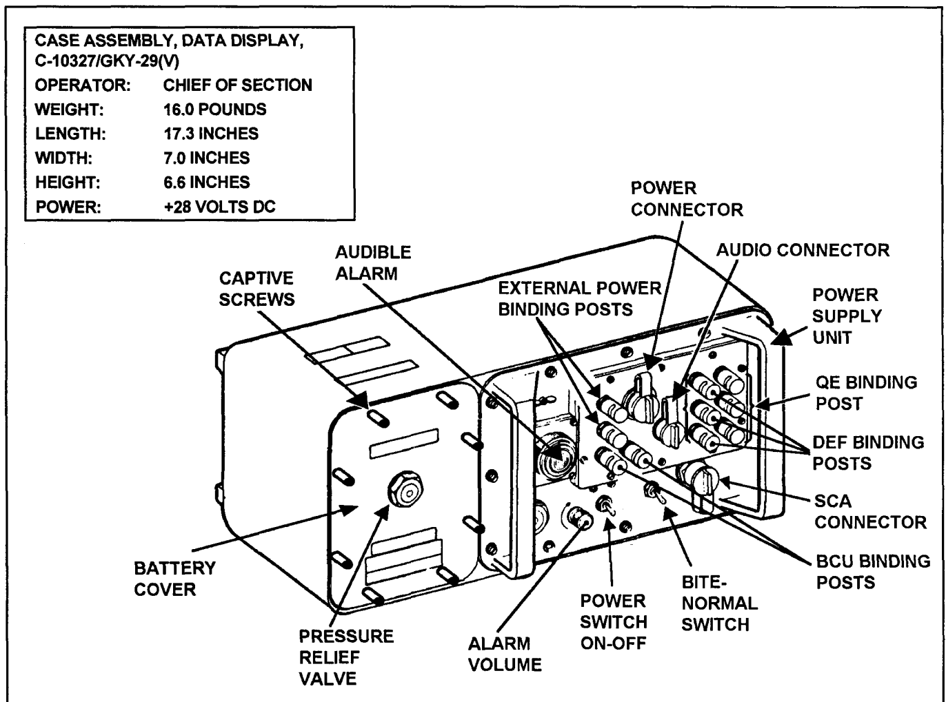
Figure L-3. Case assembly
