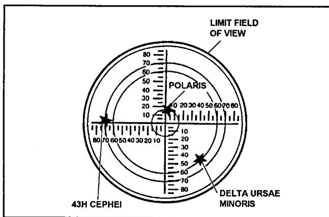
Figure 5-4. Polaris 2 with stars in tangent
