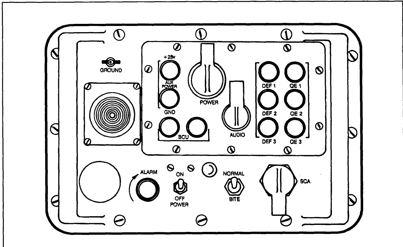
Figure L-4. Case assembly controls, indicators, and connectors
