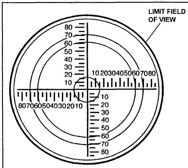
Figure 4-1. Polaris 2 reticle pattern
