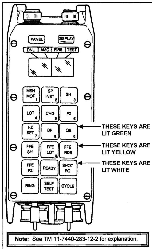
Figure L-2. Section chief's assembly controls, indicators, and connectors
