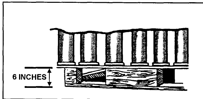
Figure 10-7. Ammunition dunnage
