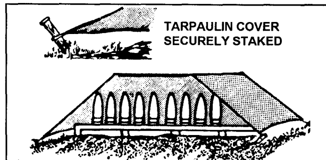
Figure 10-8. Ammunition protection
