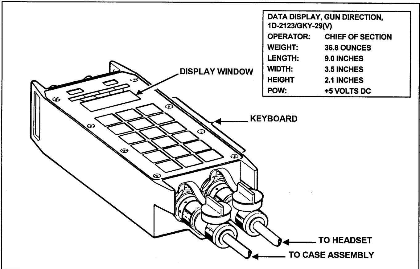
Figure L-1. Section chief's assembly
