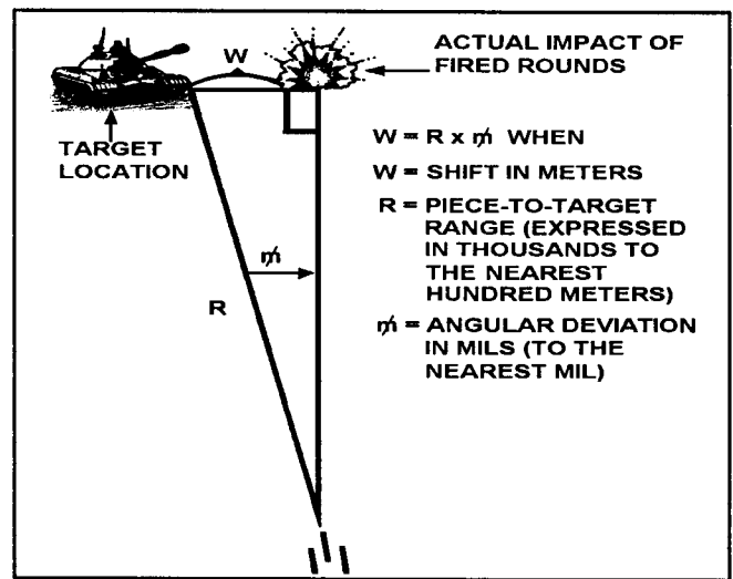
Figure D-3. Mil relation formula
