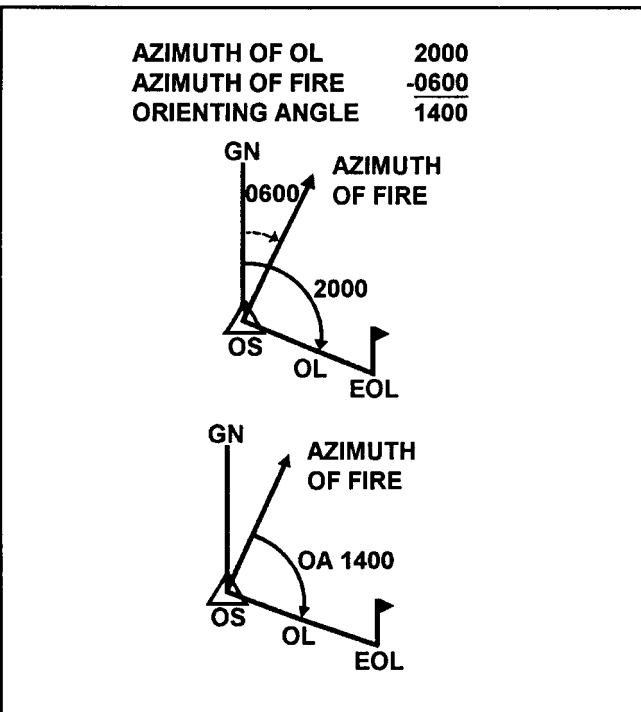
Figure 4-15. Computation of orienting angle
