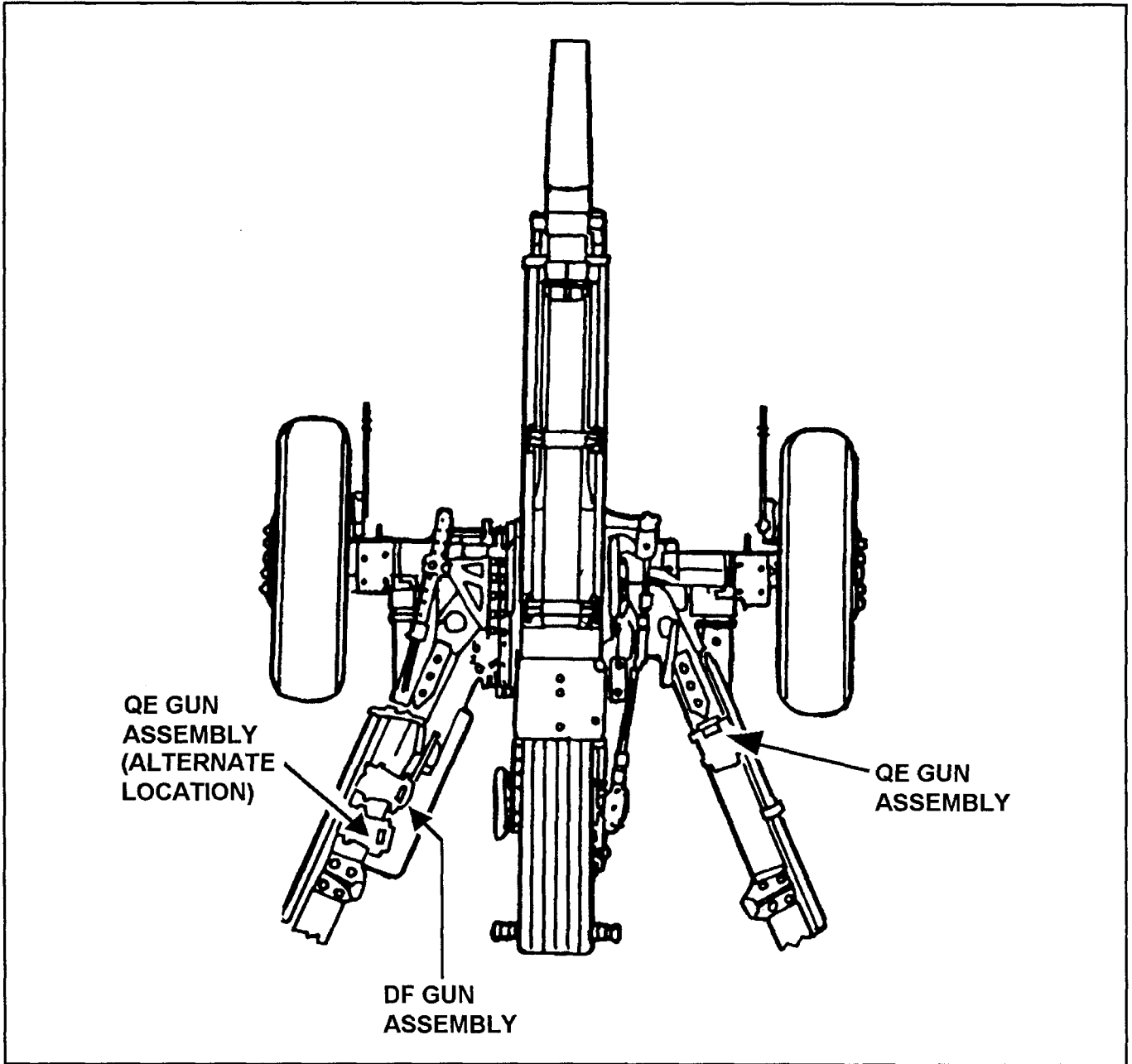
Figure L-11. Gun assemblies on M101A1 105-mm howitzer
