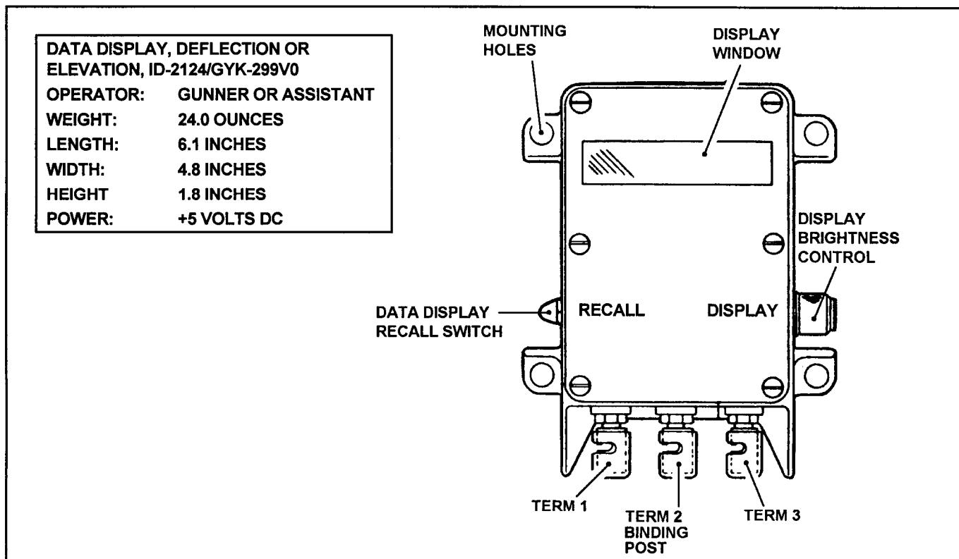
Figure L-5. Gun assembly
