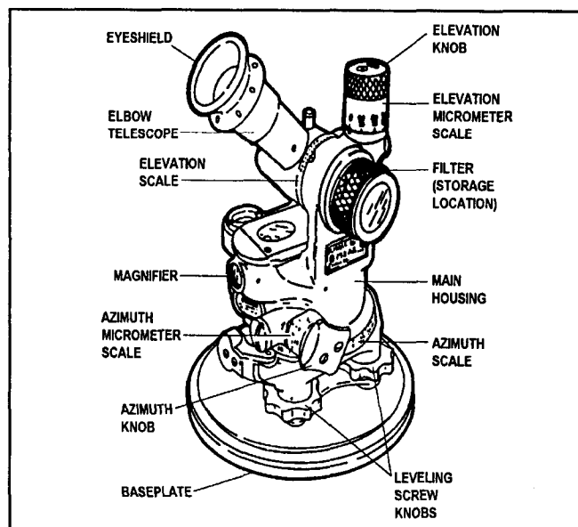
Figure 4-3. Aiming circle (right side view)
