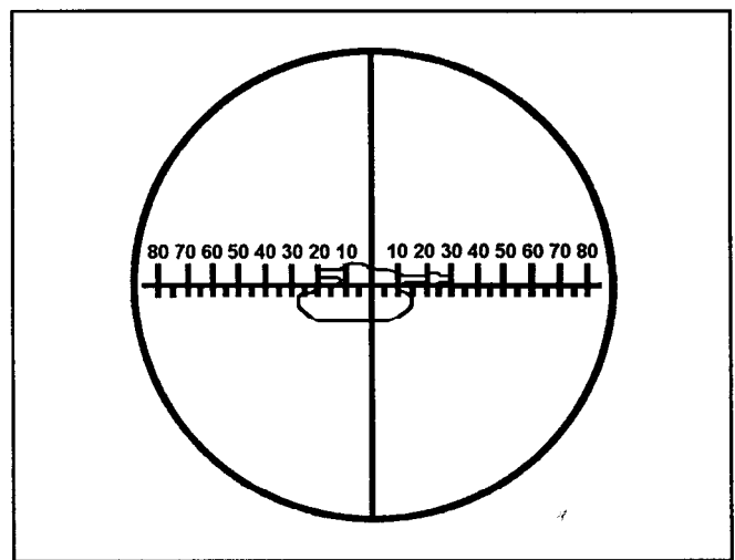
Figure 8-2. Gunner's sight picture, central laying (lead R20, deflection 3180)
