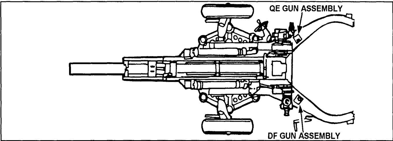
Figure L-12. Gun assemblies on M102 105-mm howitzer
