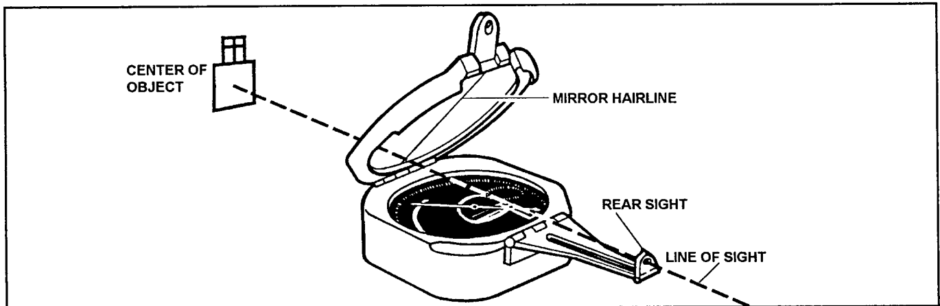
Figure 4-11. M2 compass, observer's view
