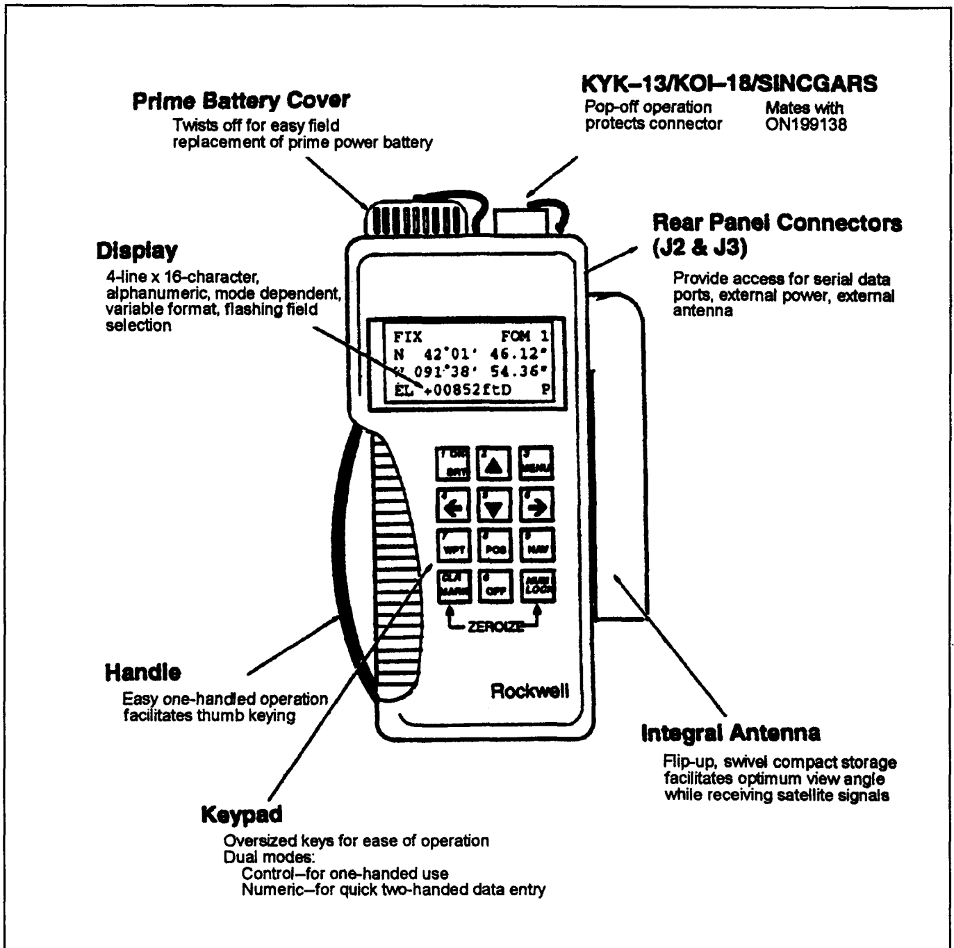
Figure 4-8. Precision lightweight GPS receiver (PLGR)
