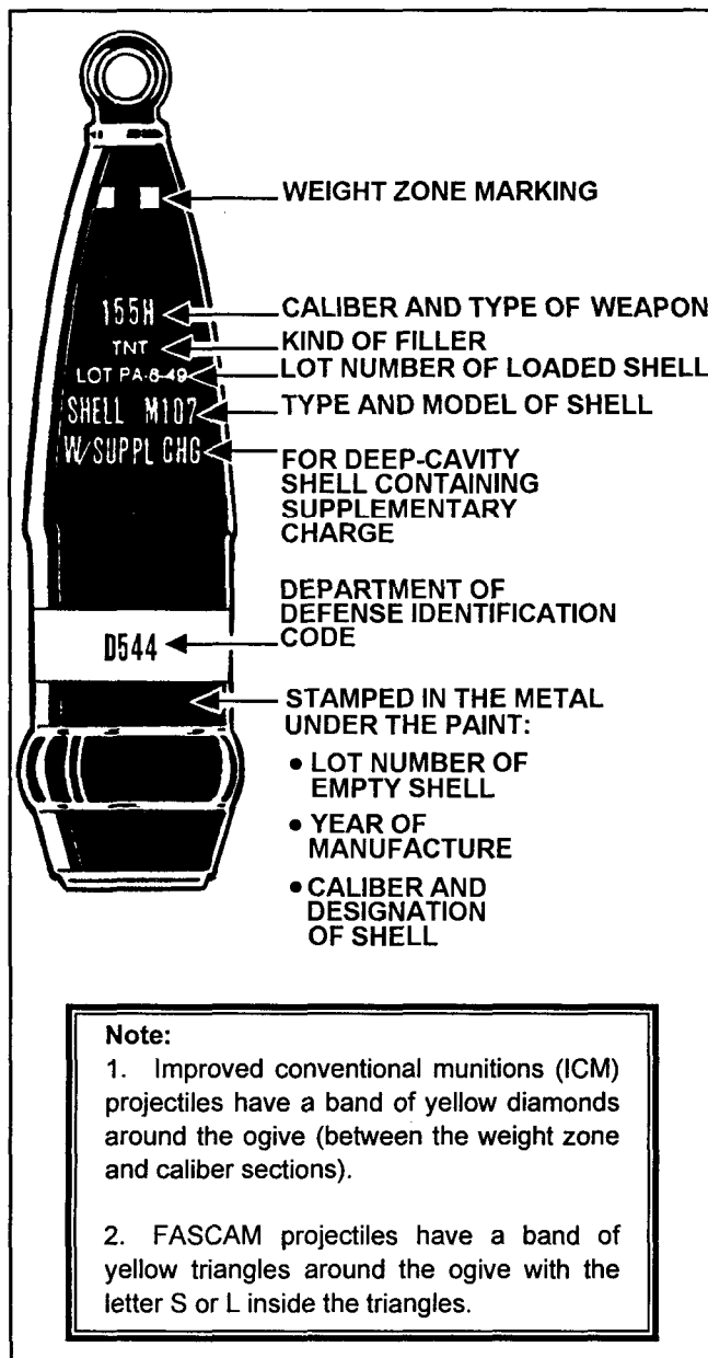
Figure 10-2. Markings of a (separate-loading) projectile
