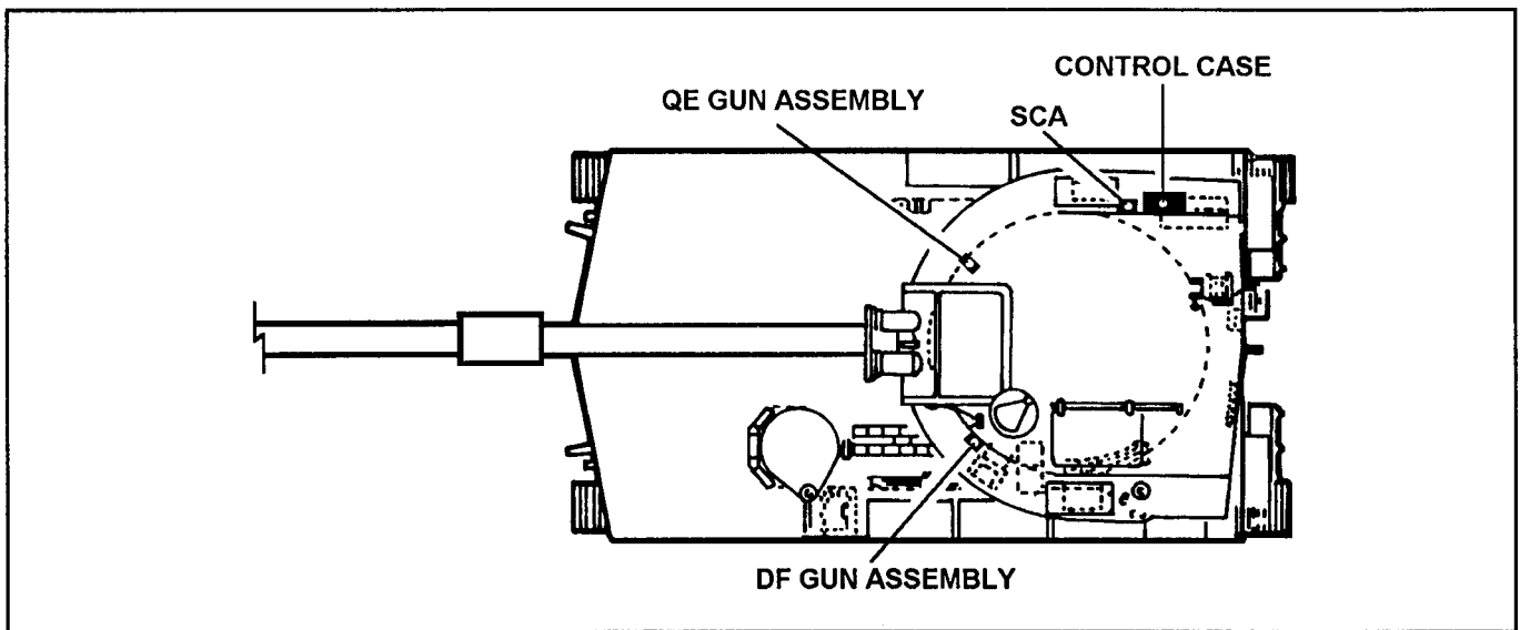
Figure L-9. GDU location on an M109-series howitzer
