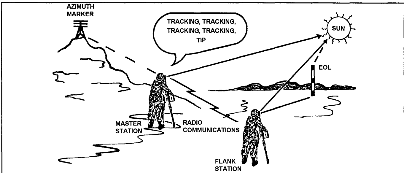
Figure 5-1. Simultaneous observation
