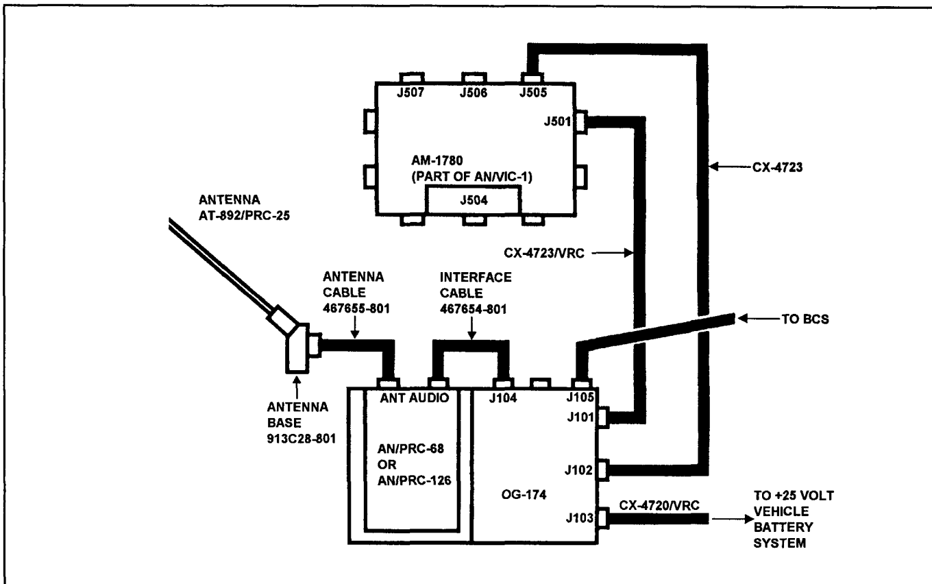
Figure 9-8. Amplifier-power supply OG-174 and small-unit transceiver AN/PRC-68 or AN/PRC-126
