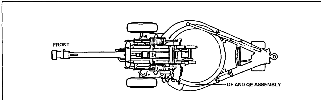
Figure L-14. Gun assemblies on M119A1 105-mm howitzer
