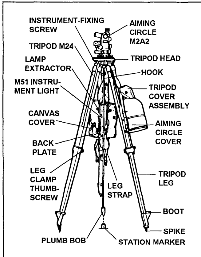
Figure 4-4. Aiming circle with tripod
