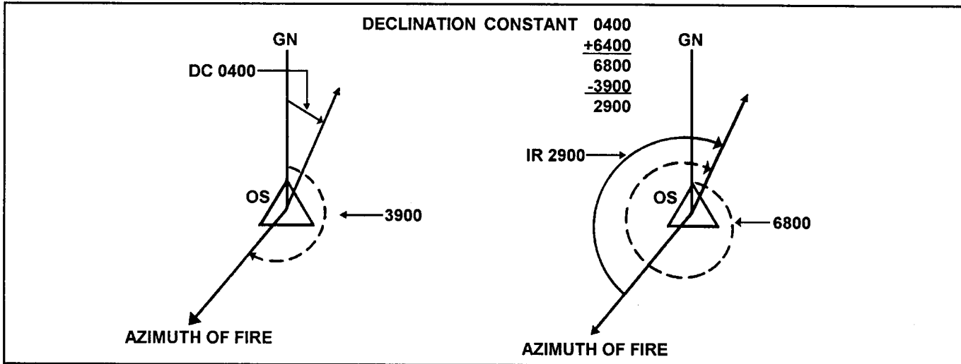
Figure 4-16. Computation of instrument reading
