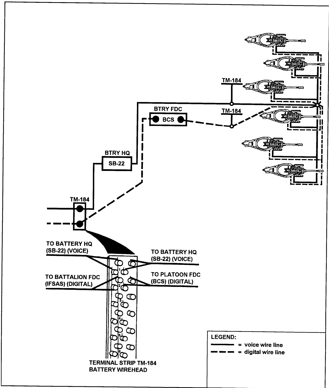
Figure 9-6. Battery-based battery wire system
