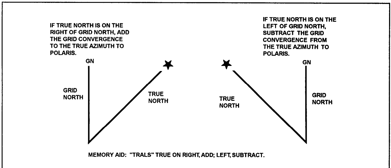
Figure 5-3. Application of grid convergence (Polaris-Kochab)
