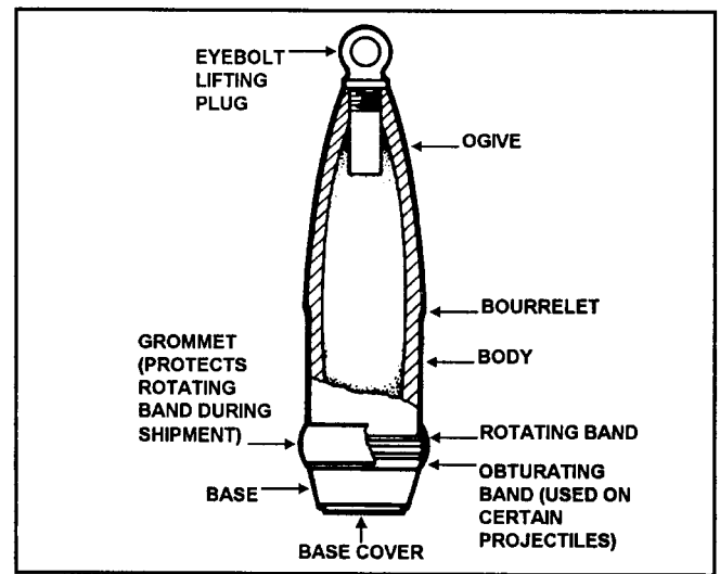
Figure 10-1. Exterior components
