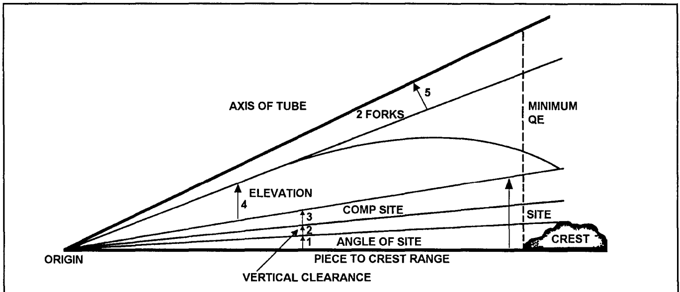
Figure 6-1. Angles in platoon leader's minimum QE
