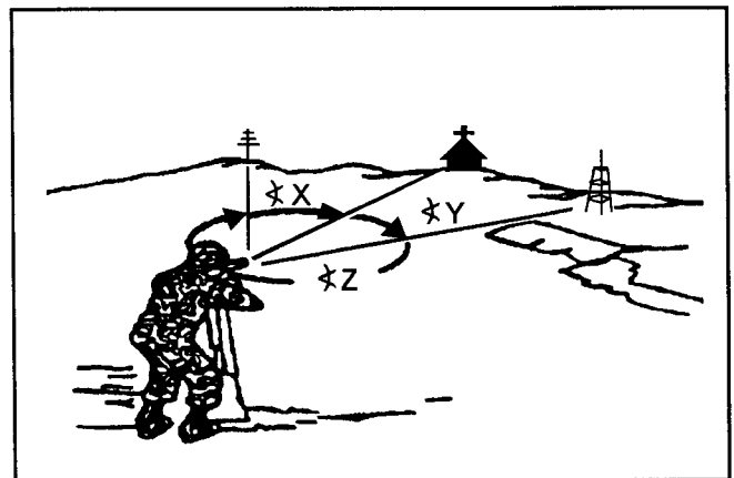
Figure 5-8. Measuring angles
