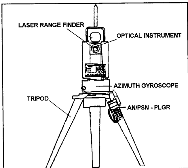
Figure 4-9. Components of the GLPS
