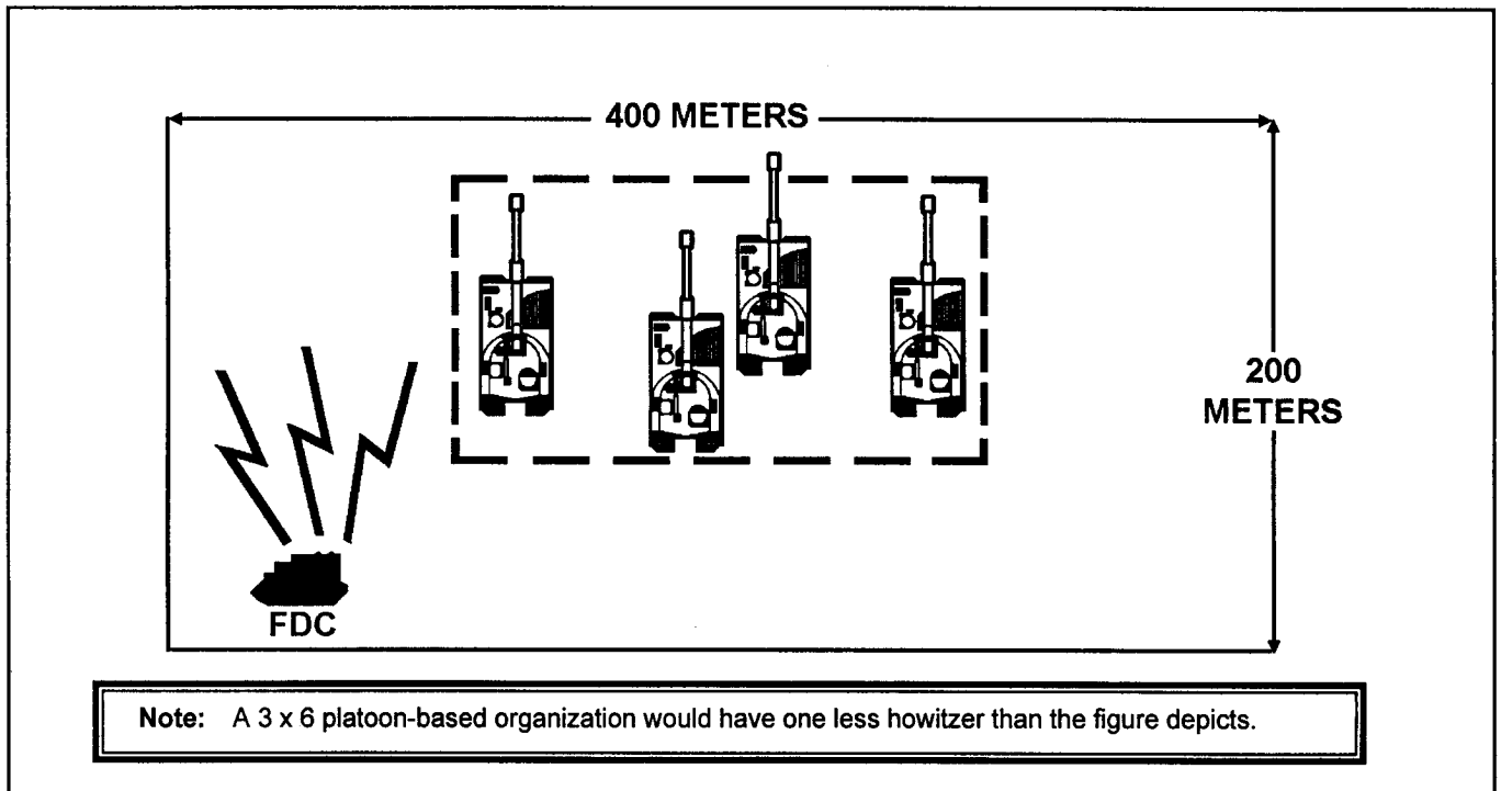
Figure 3-1. Platoon position, elements not dispersed
