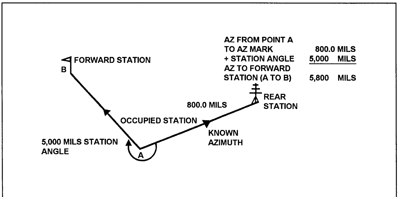
Figure 5-6. Fieldwork requirements for directional traverse
