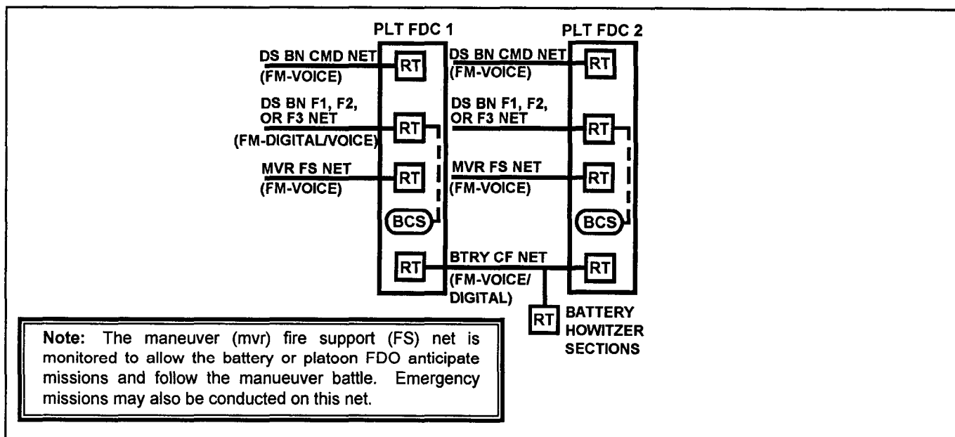
Figure 9-7. Battery radio nets
